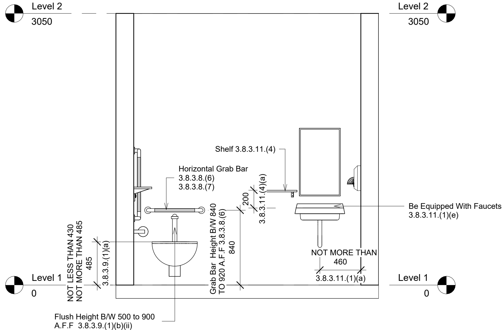
2 North Elevation 1 : 25
