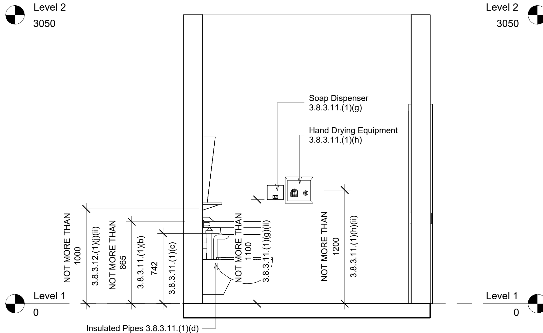
1 East Elevation 1 : 25
