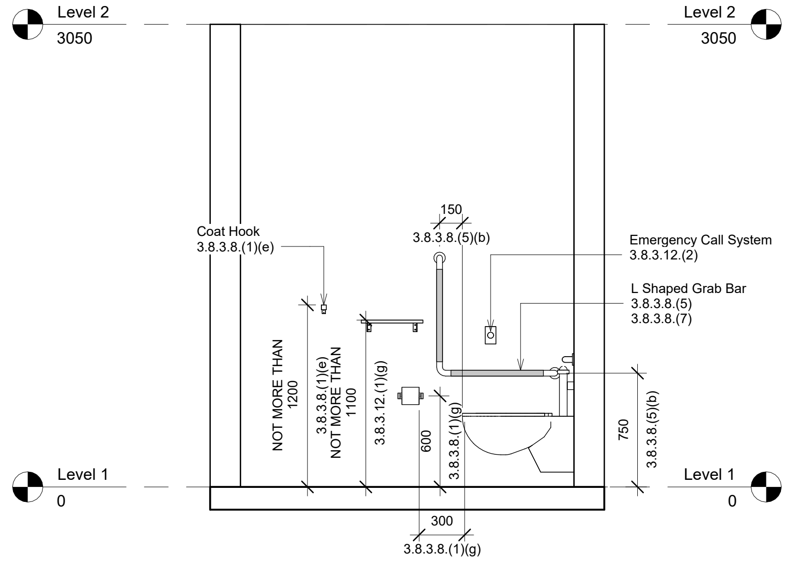
3 West Elevation 1 : 25
